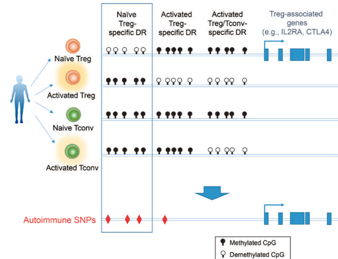
Figure 1. Autoimmune SNPs are enriched in naïve Treg cell-specific CpG hypomethylated regions. Single-nucleotide polymorphisms (SNPs) associated with common autoimmune diseases were predominantly enriched in CpG demethylated regions (DRs) specifically present in naïve Treg cells but much less enriched in activation-induced DRs common in Tconv and Treg cells. Adapted from Ohkura, Yasumizu et al., Immunity , 2020.
