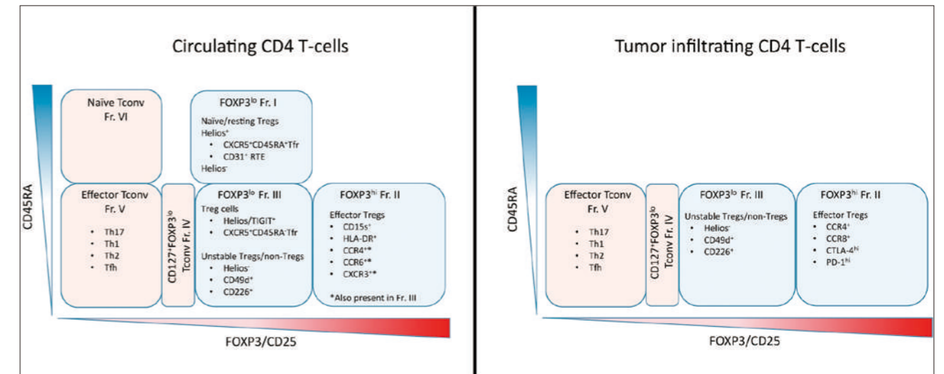
Figure 1. Main Treg Subgroups Present in Human Blood and tumors (Wing et al. Immunity 2019)
