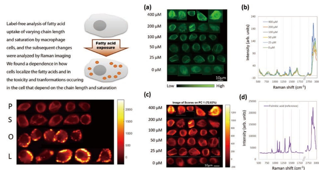
Figure 1. Uptake of palmitic acid observed in Raw264.7 macrophage cells. We compared the uptake of four different fatty acids (Palmitic, Steric, Oleic and Linoleic), and evaluate the transitions occurring in the macrophage. Changing the type of fatty acid, by varying the chain length and degree of saturation, affects the amount of uptake, the uptake timeline and the later recovery from exposure. Raman images were acquired at different concentrations, fatty acid type, and different time points. Panel (a) shows the Raman intensity (area under the curve between 2876 - 2891 cm -1 ) of five macrophage cells exposed to different concentrations of palmitic acid for 24 hours, (b) shows the average Raman spectra extracted from a 10 x 10 pixel block from all cells for each concentration of palmitic acid used and a reference Raman spectrum of palmitic acid, (c) PCA scores images for PC1 and PC2 for cells exposed to palmitic acid and (d) the reference spectra for purified palmitic acid aids the interpretation of the signals found in the macrophage cell. The five cells shown here are representative of the larger datasets collected for all cells per condition. From: Sugiyama et al. Analyst , 2020.
