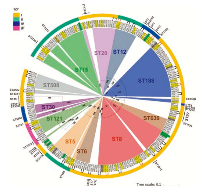
Figure 2. Whole-genome sequencing of S. aureus strains isolated from the skin of Japanese infants.
