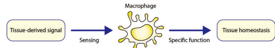
Figure 2. Macrophages are essential components for the maintenance of tissue homeostasis.
