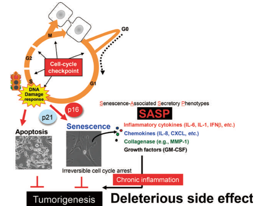
Figure 1. Cellular senescence initially inhibits proliferation of damaged cells, thereby acting as a fail-safe mechanism. However, in the long term, senescent cells eventually promote tumorigenesis via SASPs.
