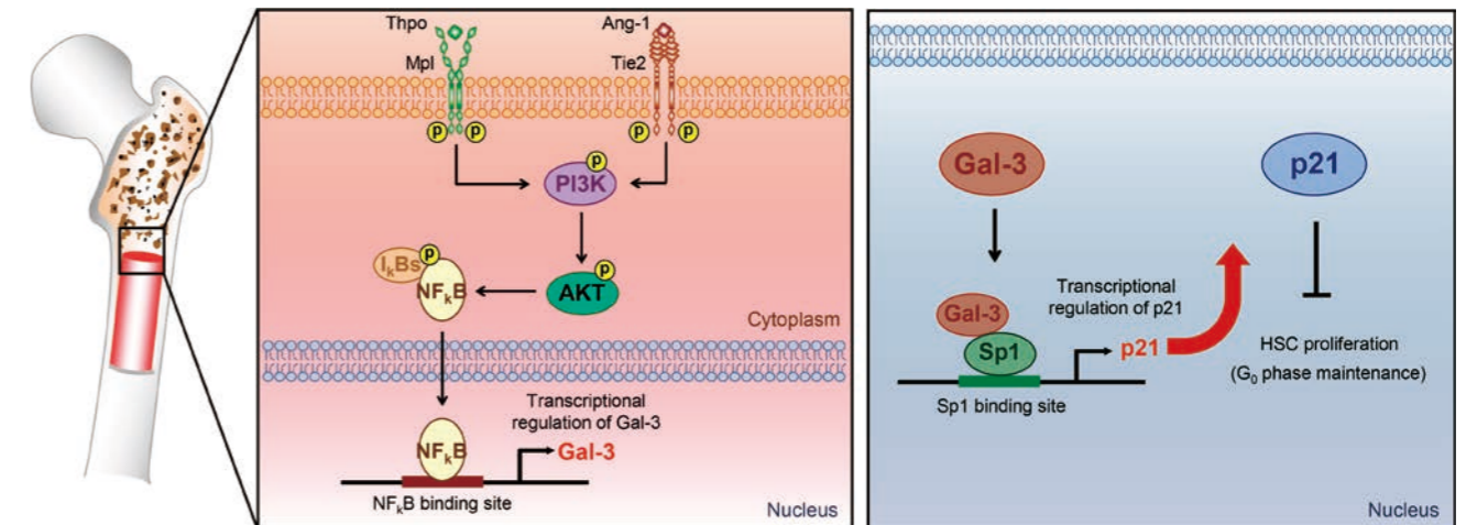
Figure. Proposed model showing the molecular mechanisms essential for maintaining (long term-hematopoietic stem cell) LT-HSC quiescence.
