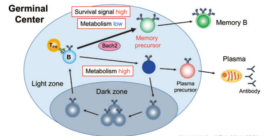
Figure. During germinal center (GC) reaction, light zone B cells are selected to differentiate into memory B cells, plasma cells, or to re-enter the dark zone. We have identified and characterized a small GC population of precursors for memory B cells, and found that the GC B cells with lower mTORC1 activity resulting from receiving weak T cell help and those with a higher survival signal from surface B cell receptors favor a memory B cell fate.
