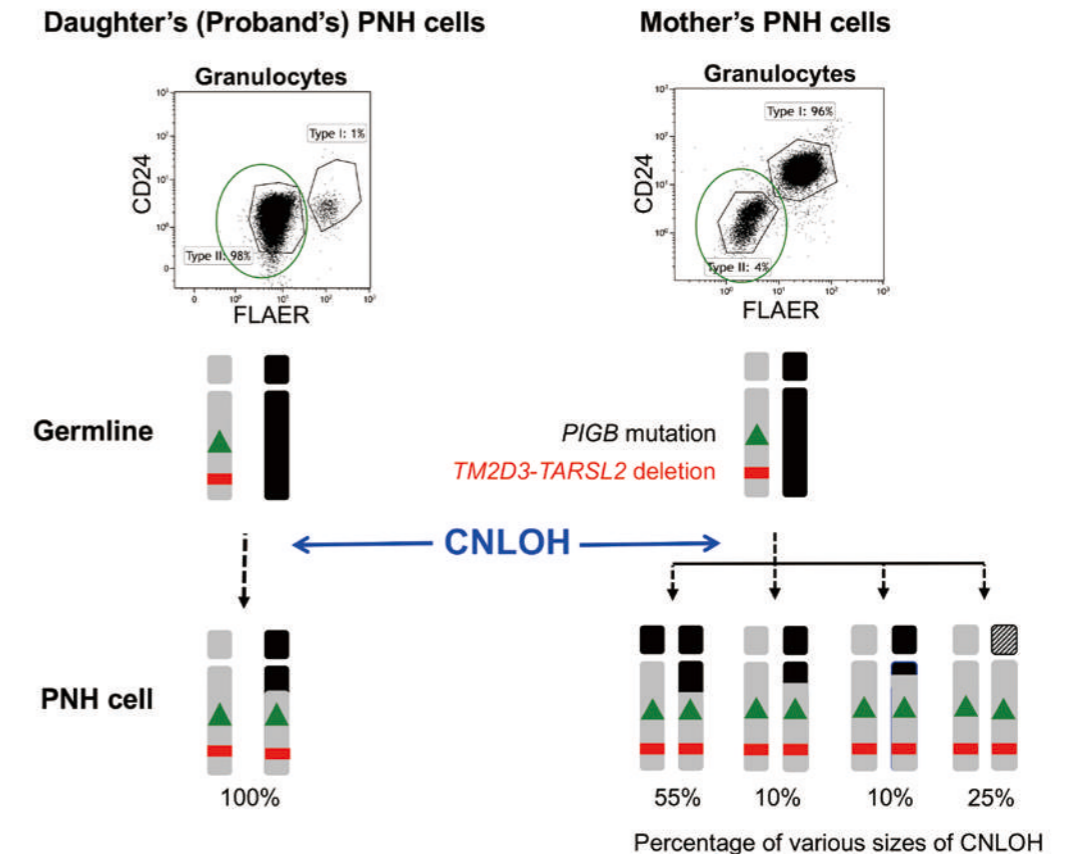
Figure 1. Germline PIGB mutation and 70kb deletion became homozygous by CNLOH. Upper: Proband's and mother's blood granulocytes contained PNH cells. Lower: One and four PNH clones with CN-LOH regions of different lengths were found in proband and mother, respectively. (Adopted from Langemeijer, S. et al, Blood Adv., 2020, 4(22): 5755-5761)
