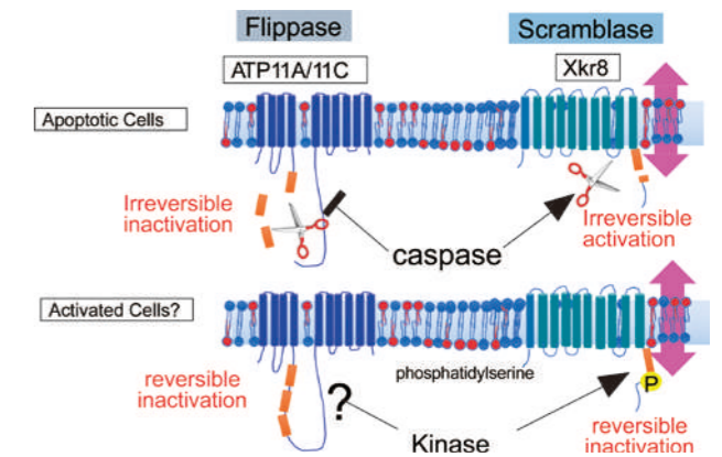
Figure 2. Activation of Xkr8's scramblase and inactivation of flippases by two independent mechanisms.
