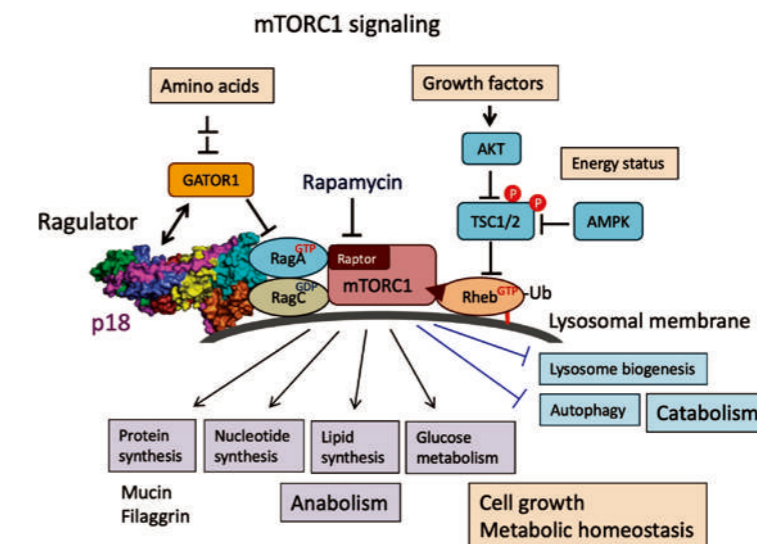
Figure 2. Function and regulation of the mTORC1 signaling on lysosomal membrane.
